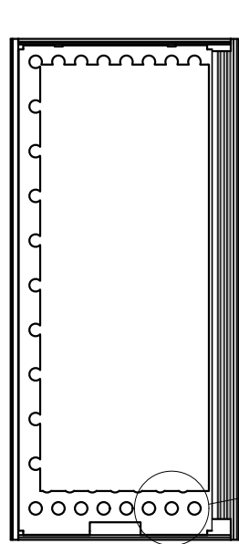
DETAIL A-A PANEL REINFORCEMENT (0.023" Thick Steel)
