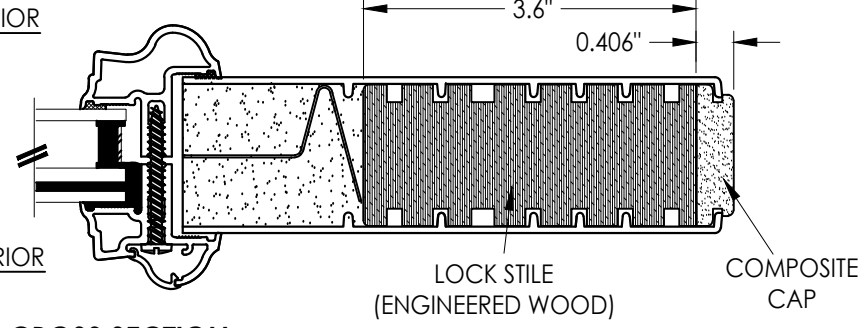
2 2 HORIZONTAL CROSS SECTION
