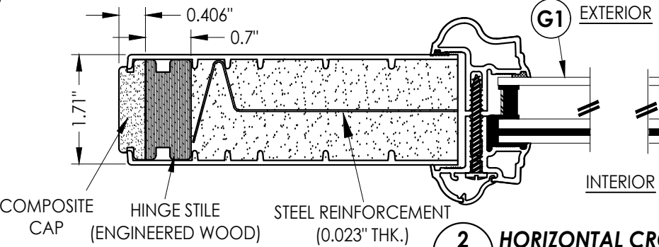
2 2 HORIZONTAL CROSS SECTION
